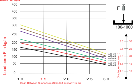
Load Graph
